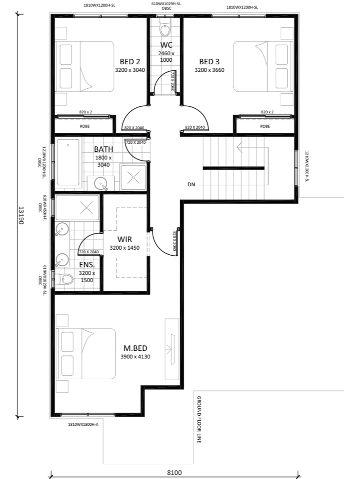
UPPER PLAN
