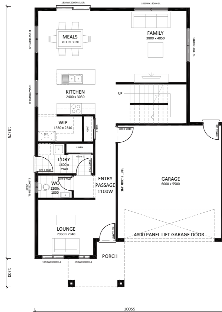
LOWER PLAN
