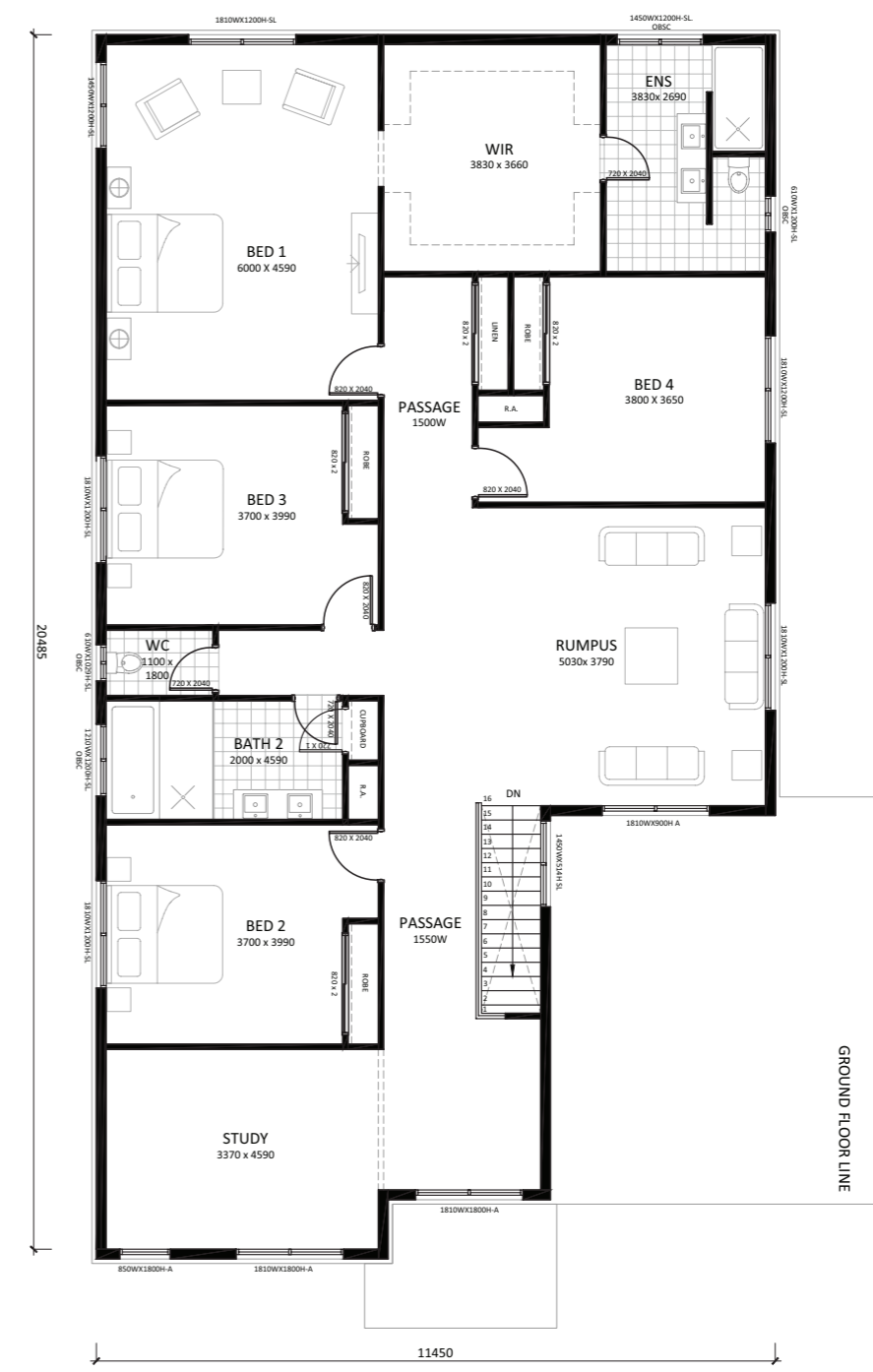
UPPER PLAN
