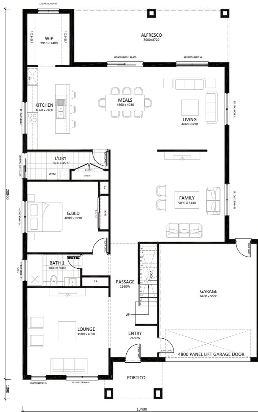
LOWER PLAN
