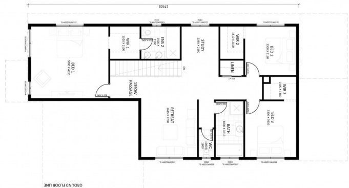
UPPER PLAN
